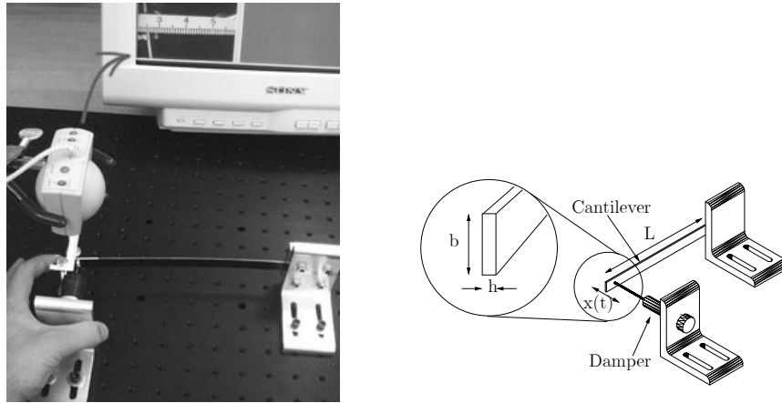
Figure 1: First-order spring-damper system
